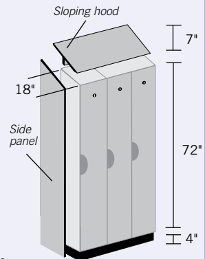
Side panel (#33334) and sloping hood (#33353) on three (3) wide single tier locker (#31368) displayed
