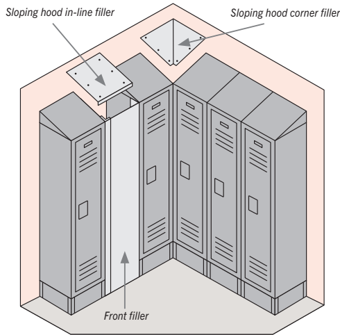
Locker installation with sloping hoods
