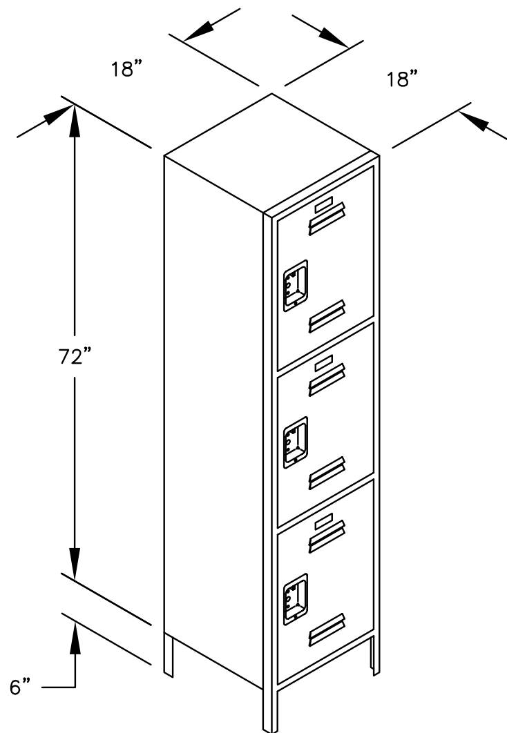
MODEL #18-53168 18" WIDE TRIPLE TIER STANDARD LOCKER – 1 WIDE
