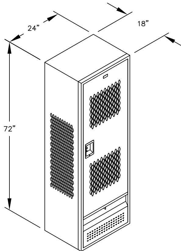
MODEL #72018 24" WIDE STANDARD GEAR LOCKER WITH VENTILATED DOOR
